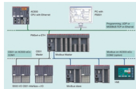
PLC
